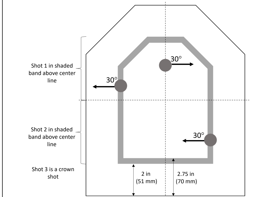
Figure 8. NIJ RF1, NIJ RF2, and NIJ RF3: Example of Shot Placement for 3 Shots per Test Item on a Multi-Curve Plate
