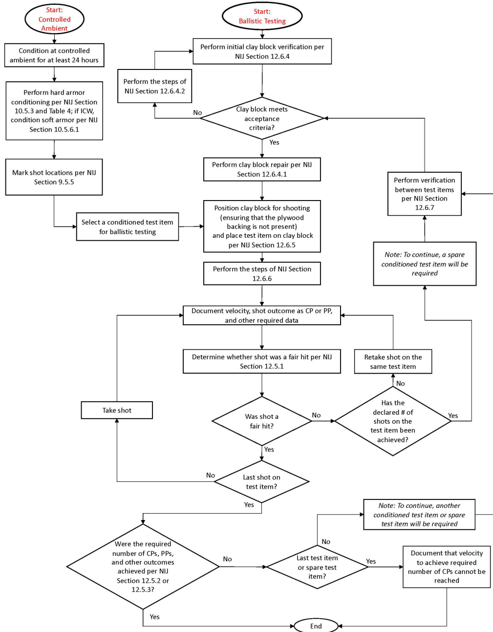
Figure H.4. Hard Armor Procedure Flowchart for Ballistic Limit Testing
