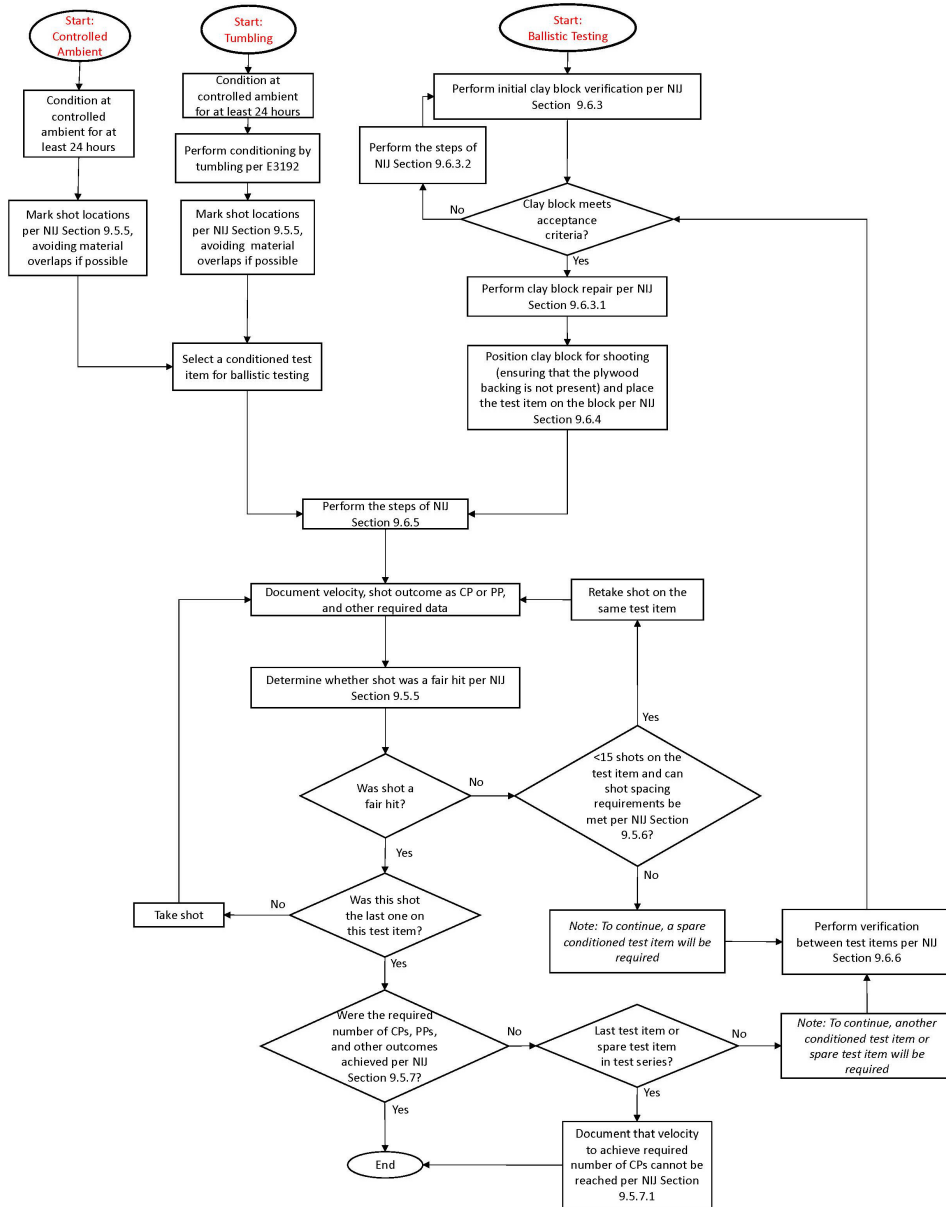
Figure H.2. Soft Armor Procedure Flowchart for Ballistic Limit Testing
