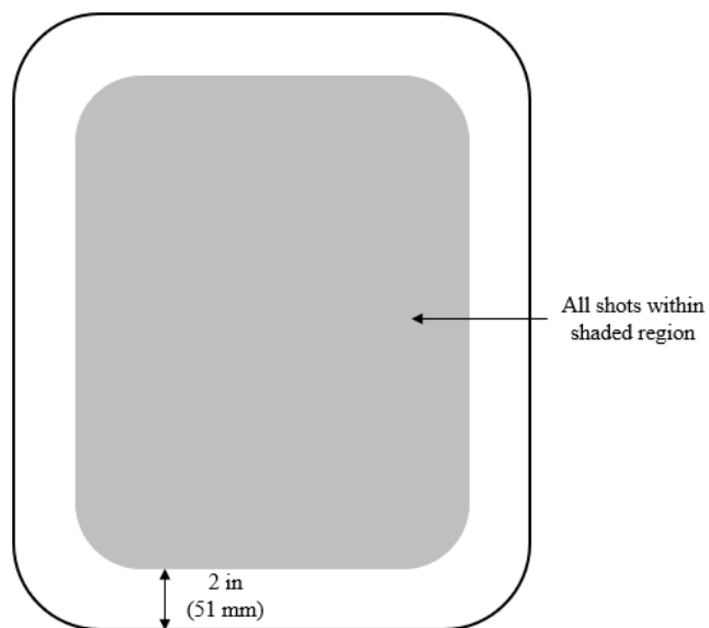
Figure 11. NIJ RF3: Shot Placement for 1 or 2 Shots Per Test Item
