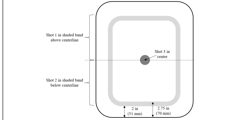
Figure 7. NIJ RF1, NIJ RF2, and NIJ RF3: Shot Placement for 3 Shots per Test Item
