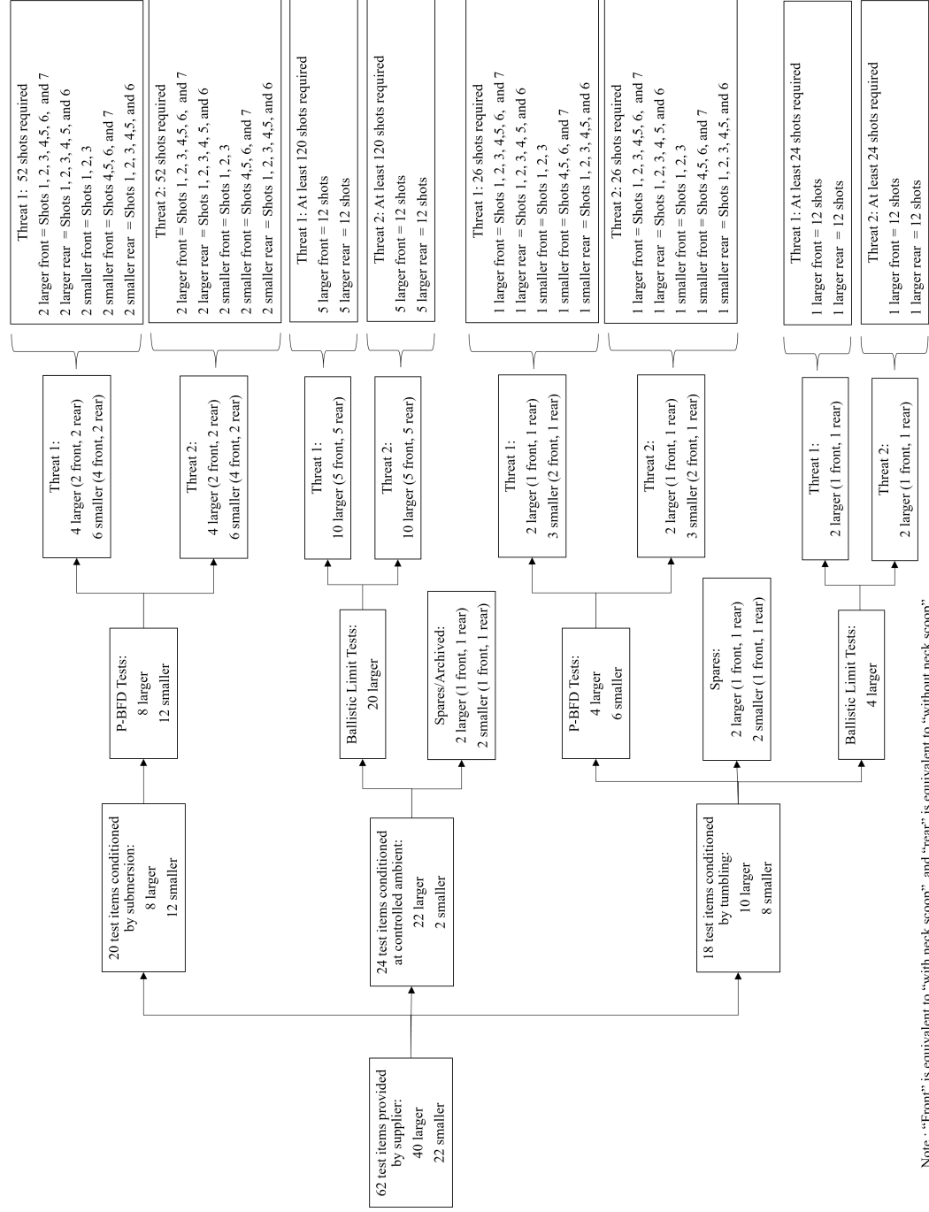
Figure 2. NIJ HG1 and NIJ HG2: Allocation and Utilization of Planar Soft Armor Test Items
