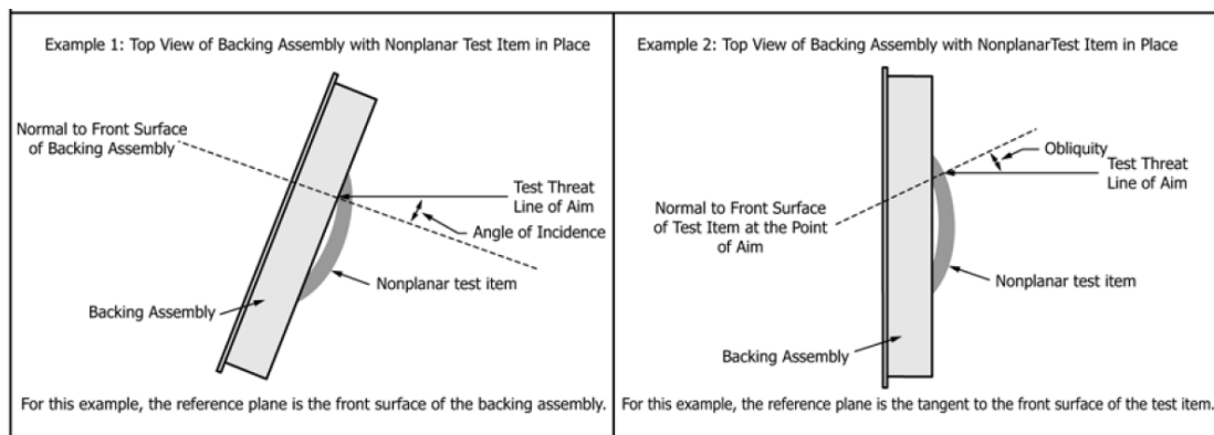
Figure 1. Examples showing angle of incidence and obliquity using a clay block backing assembly
