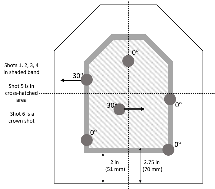
Figure 10. NIJ RF1, NIJ RF2, and NIJ RF3: Example of Shot Placement for 6 Shots Per Test Item on a Multi-Curve Plate
